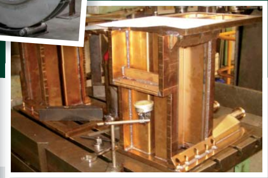
Precision fabrication and CNC machining of superior filler heads for cheese.
